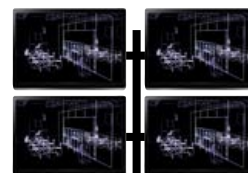
System 4
