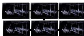
System 6
