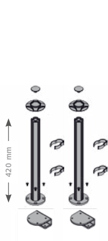
436-FP42 2 poles with clips and desk mount. Bracket, max. table top 25 mm.
